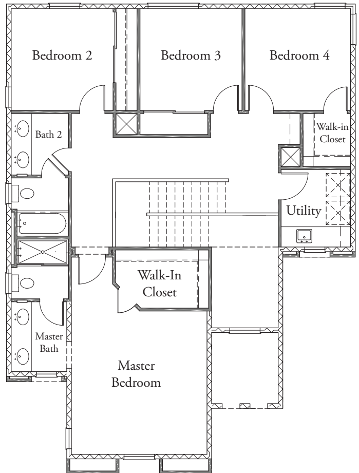
Second Floor
